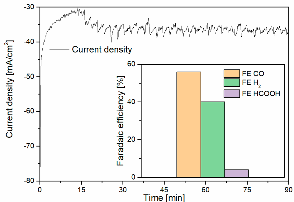
Figure 8. Conversion module results with an initial 50%/50% gas stream; average current density during the measure and (inset) faradaic efficiencies of the reaction products (FE = faradaic efficiency).
