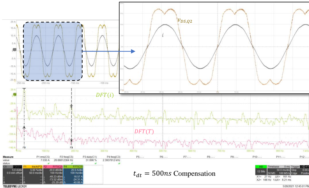
Fig. 12: Motor current in the time domain and DFT of phase current and machine mechanical torque 50 ms/div. t_{at} = 500\text{ ns} with compensation algorithm. C5: motor phase current i 5 A/div. F1: reconstructed inverter voltage v_{DS,Q2} 5 %/div. F2: DFT of the mechanical torque 500 mV/Nm. F4: DFT of the inverter phase current.
