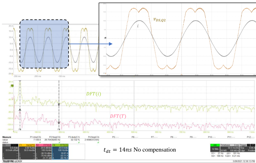
Fig. 13: Motor current in the time domain and DFT of phase current and machine mechanical torque 50 ms/div. t_{at} = 14\text{ ns} with no compensation algorithm. C5: motor phase current i 5 A/div. F1: reconstructed inverter voltage v_{DS,Q2} 5 %/div. F2: DFT of the mechanical torque 500 mV/Nm. F4: DFT of the inverter phase current.
