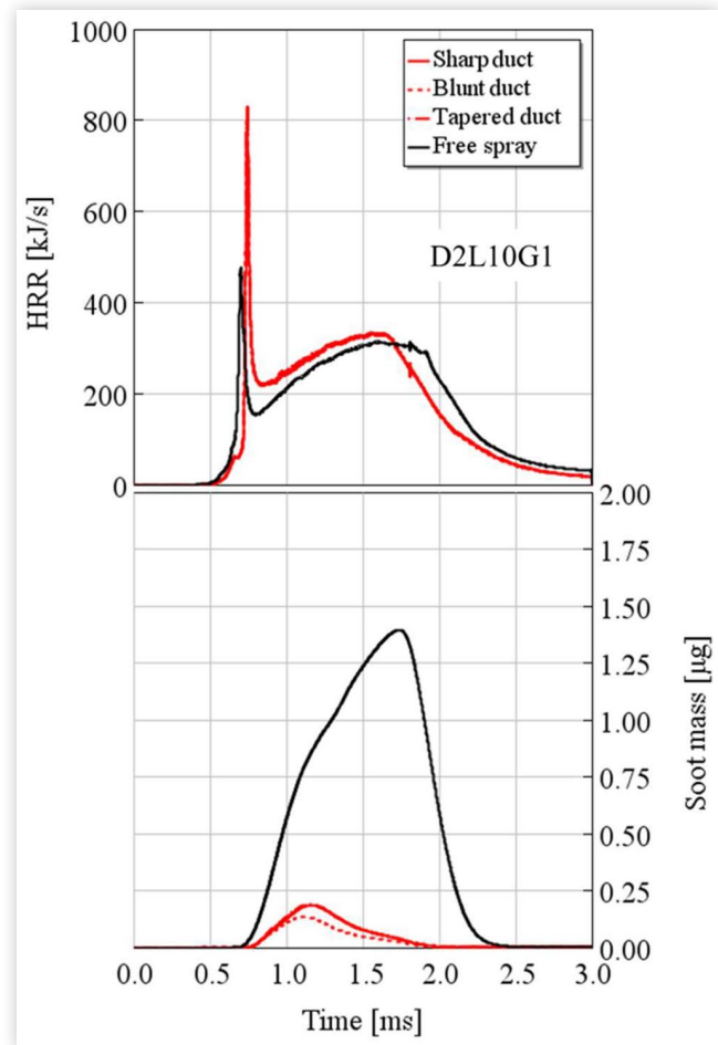
FIGURE 27 HRR (top) and soot mass in the CVV (bottom) as a function of time for the free-spray (black) and three different duct shapes (D2L10G1 geometry), defined in Figure 6: sharp duct (red, continuous line), blunt duct (red, dotted line), tapered duct (red, dashed line). Operating conditions: vessel pressure = 57.3 bar; vessel temperature = 900 K; rail pressure = 1200 bar.
