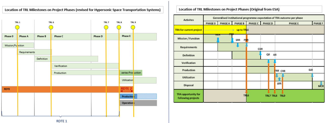
Figure 5 Location of TRL Milestones on Project Phases: original ESA subdivision [26] (right) vs. revised version for hypersonic
