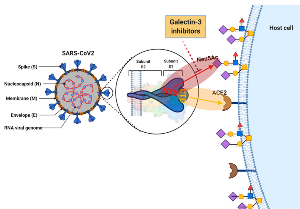
Figure 4. A dual attachment model for SARS-CoV2. This shows that a pocket in the NTD of SARS-CoV2 is capable of binding N -acetylneuraminic acid (Neu5Ac) [25] and strongly supports a dual attachment model for SARS-CoV2, where NTD-Neu5Ac interactions facilitate initial host cell recognition by the virus and stabilise its entry via ACE2 receptors. Adopted from [13] with permission.
