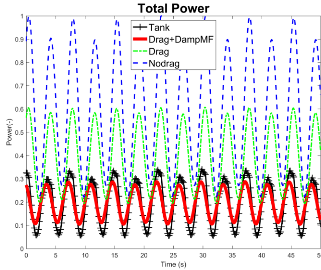
Figure 13: Total normalized power at a full scale of the tank testing and the 3 numerical models: the drag + mechanical friction, the drag and the no-drag model. (Single column image)
