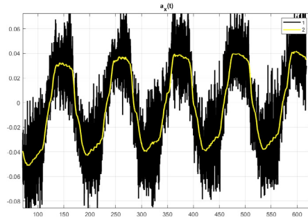
Fig. 8. Filtered acceleration
