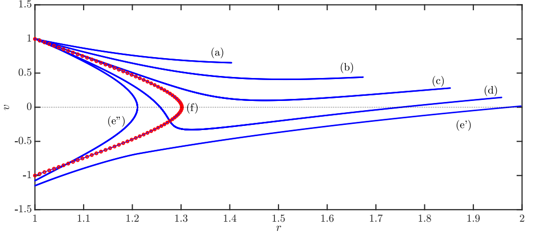
FIGURE 3. Phase-space evolution for the electron distribution in the same case of Fig. 1. The different curves a,b,c,d,e'-e'', f, correspond to different times t = 0.5, 1, 1.5, 2, 2.5, 100 . The steady-state solution (from system (2.7)) is also presented (circles).
