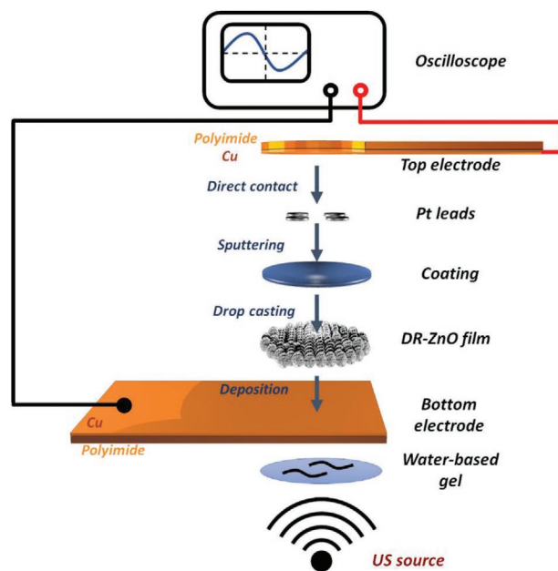
Figure 13. Schematics of the DR-ZnO films electromechanical characterization setup.
