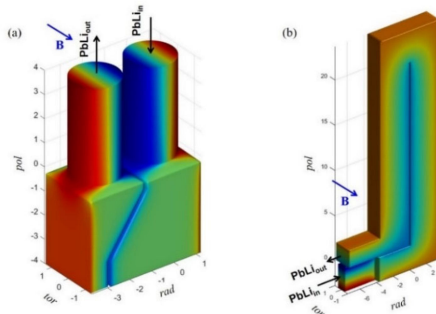
Figure 2. Examples of application of asymptotic methods for the study of pressure-driven MHD flows in (a) a DCLL geometry proposed in [16] and in (b) a model geometry for a modular DCLL, as shown in [17]; contours of electric potential are plotted on the fluid–wall interfaces.
