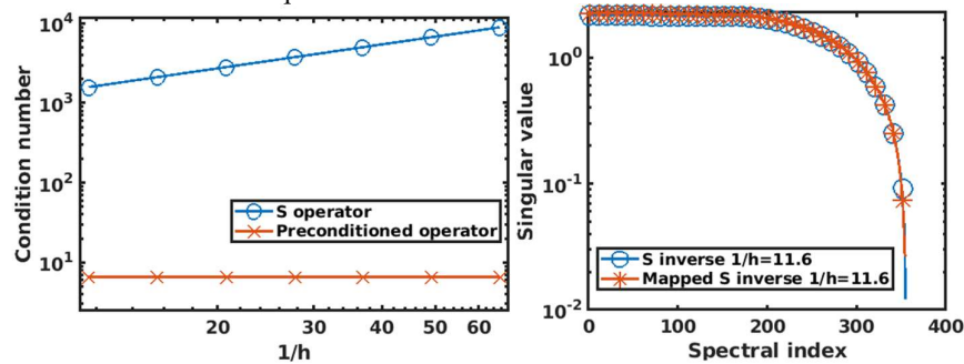
Figure 1. Left: condition numbers of \mathcal{S}_{\lambda,\lambda} and \tilde{\mathcal{P}}_{\tilde{\lambda},\tilde{\lambda}} (\mathbf{G}_{\lambda,\lambda})^{-1} \mathcal{S}_{\lambda,\lambda} . Right: spectra of \tilde{\mathcal{P}}_{\tilde{\lambda},\tilde{\lambda}} and \mathbf{G}_{\lambda,\lambda} (\mathcal{S}_{\lambda,\lambda})^{-1} \mathbf{G}_{\lambda,\lambda} .
