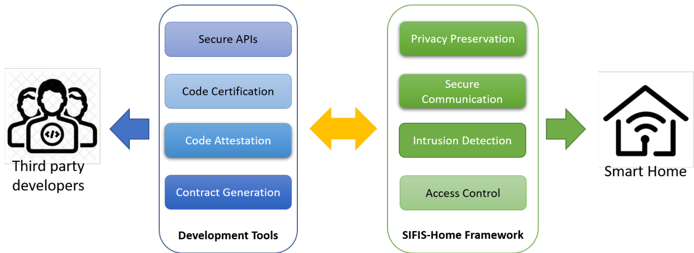
Fig. 1: The SIFIS-Home software components.
