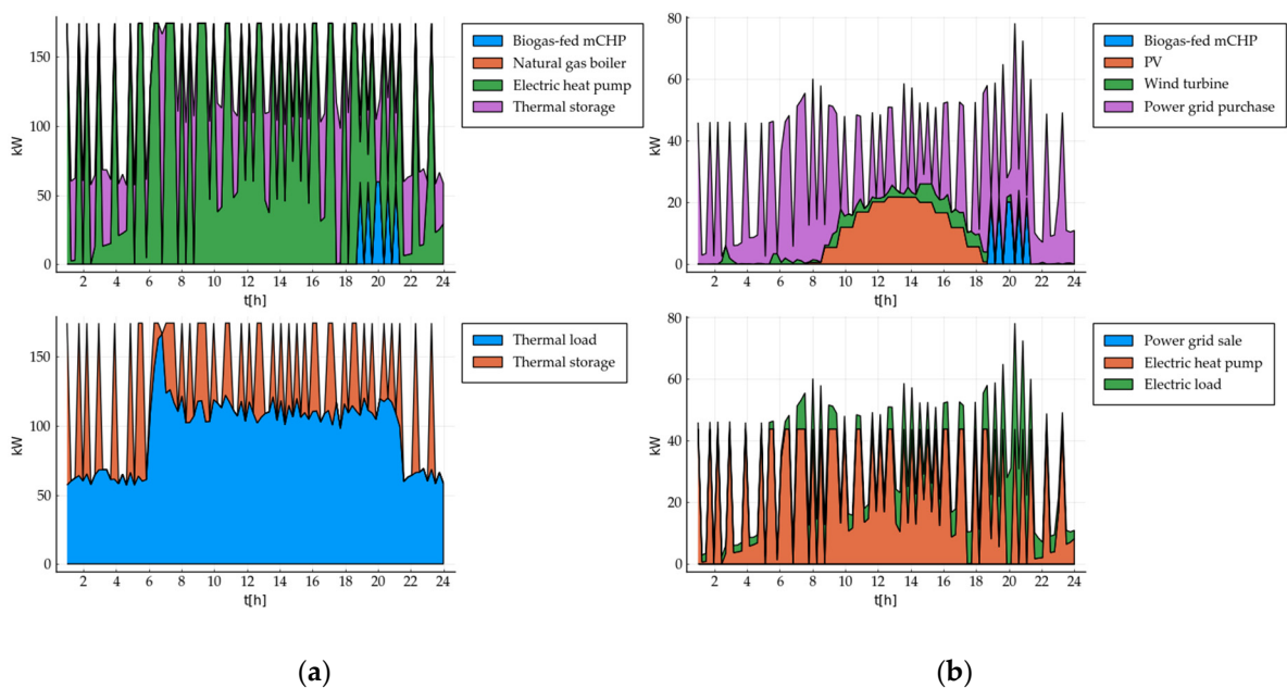
Figure 12. Daily consumption and production pattern for Case 1 (Operation Optimization) with a biogas price of 0.39 \text{ €/m}^3 : thermal production (a-up) consumption (a-down); electricity production (b-up) consumption (b-down).
