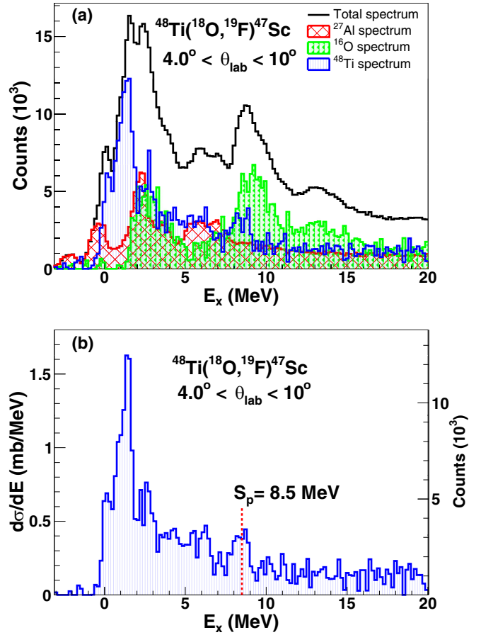
FIG. 7. (a) Decomposition of the excitation energy spectrum obtained with the \text{TiO}_2 + ^{27}\text{Al} target. The total spectrum is presented with the solid black line. The red-hatched area corresponds to the normalized background originating from the ^{27}\text{Al} backing material, while the dotted green area corresponds to the background arising from oxygen. The blue vertically hatched area is the obtained excitation energy spectrum for the ^{48}\text{Ti}(^{18}\text{O}, ^{19}\text{F})^{47}\text{Sc} reaction, after subtracting from the total spectrum the background contributions. (b) Reconstructed excitation energy spectrum for the ^{48}\text{Ti}(^{18}\text{O}, ^{19}\text{F})^{47}\text{Sc} reaction at 275 MeV. The proton emission threshold of ^{47}\text{Sc} nucleus is indicated with the vertical red dashed line.
