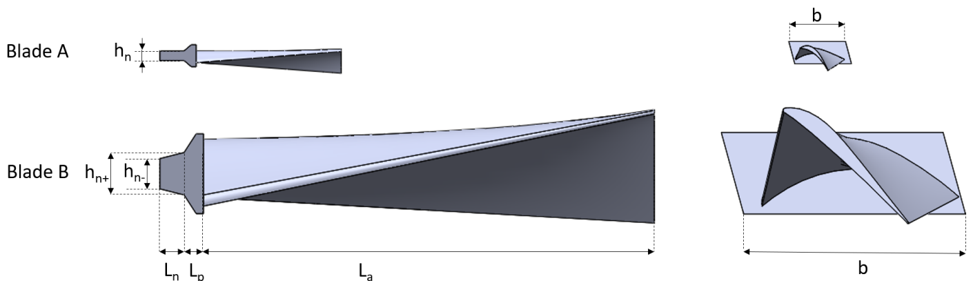
Figure 9. CAD model front and top view of the two blades investigated with this paper. The figure indicates proportions, and the values for symbols are shown in Table 2.
