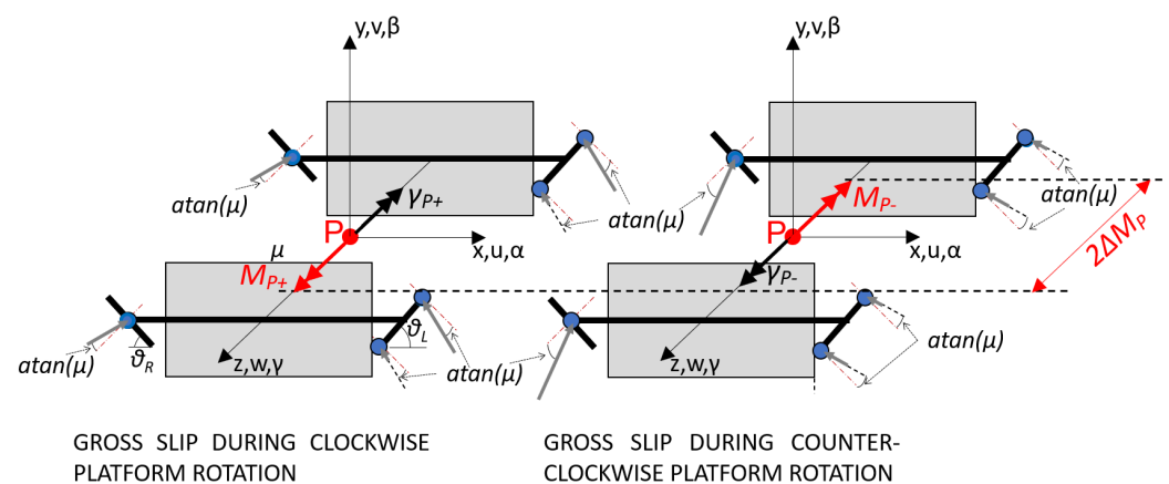
Figure 7. Representation of contact forces and their moments about platform point P for an In-Phase mode of vibration.
