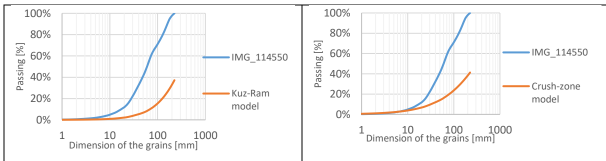
Figure 3. Comparison between the particle size distributions obtained with Split Desktop and those from Kuz-Ram and Crush-zone models.
