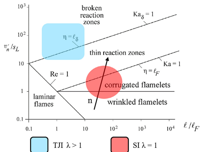
Fig. 3. Representation of expected combustion regimes on Borghi's diagram [29] for lean burn TJI engines (light blue area) and conventional homogeneous charge SI engines (red area). (For interpretation of the references to color in this figure legend, the reader is referred to the web version of this article.)
