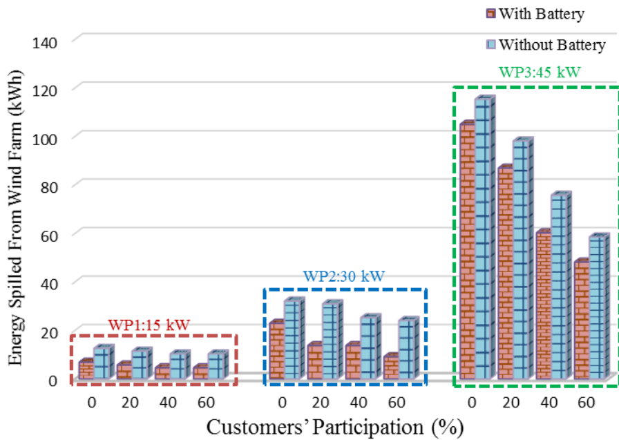
Fig 11: Spilled wind power with considering battery
