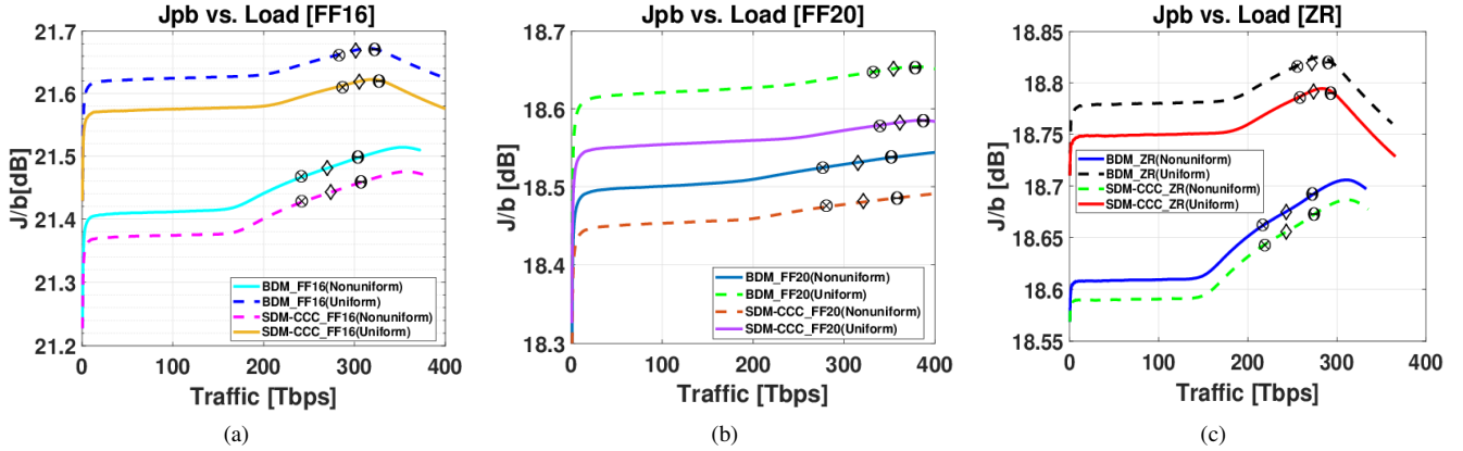
Fig. 2: Energy consumption per bit – as dB Joule per bit – versus total allocated traffic for (a) FF16, (b) FF20 and (c) ZR TRXs for SDM and BDM with uniform and nonuniform JPFD traffic distribution in COST topology. \otimes , \diamond and \ominus identify the BP of 0.1%, 1% and 10%, respectively.
