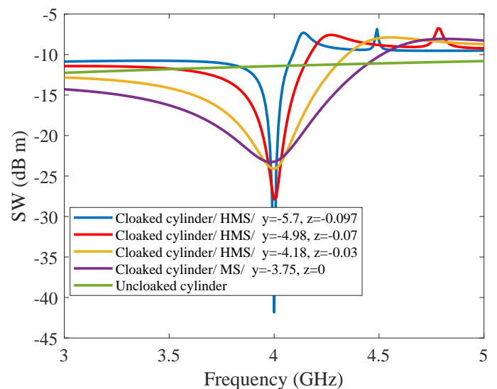
Fig. 3: SW of a PEC cylinder with a radius of b = 0.06\lambda_0 and a dielectric spacer with relative permittivity of \epsilon_r = 10.2 and thickness of 1.27324 mm covered by a proper conformal HMS.
