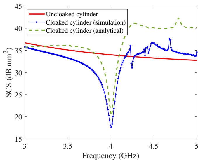
Fig. 7: Comparison of SCS of the uncloaked and cloaked conducting cylinders.
