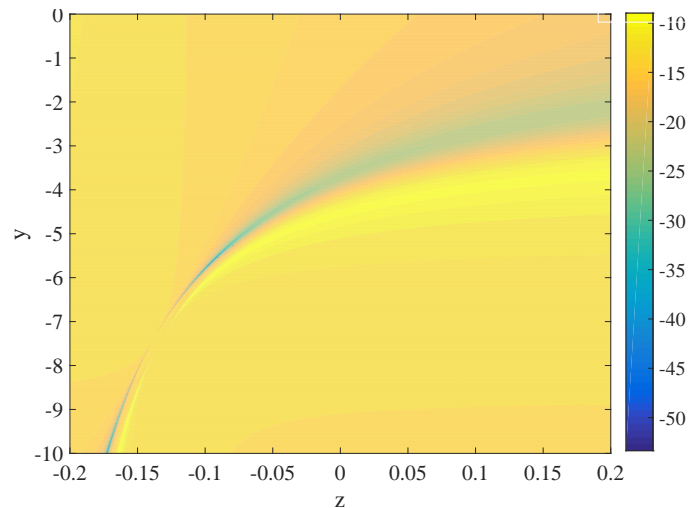
Fig. 2: SW (dB) with respect to varying y = (j\eta_0 Y_{es})/2 and z = Z_{ms}/(2j\eta_0) corresponding to the HMS at 4 GHz.
