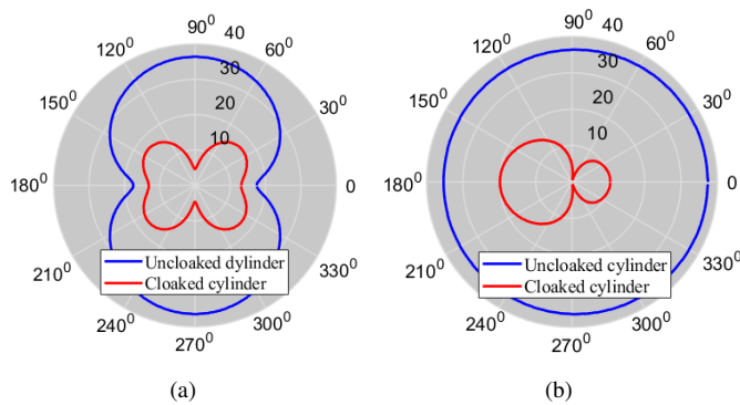
Fig. 10: SCS ( \text{dBmm}^2 ) polar plot of cloaked and uncloaked cylinders for (a) \phi = 90^\circ , and (b) \theta = 90^\circ .
