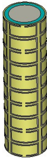
Fig. 6: The conducting cylinder covered by a Huygens' metasurface.
