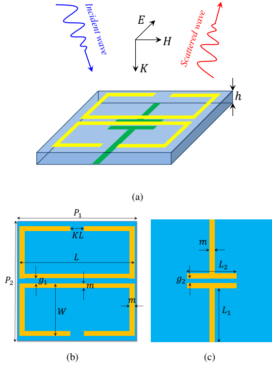
Fig. 4: Geometry of the proposed planar HMS unit cell (a) 3-D view, (b) top layer, and (c) bottom layer.
