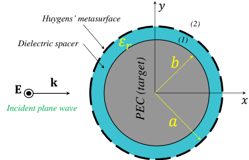
Fig. 1: Schematic geometry of a PEC cylinder and dielectric spacer covered by a conformal HMS, illuminated by a normally incident TM-polarized plane wave.
