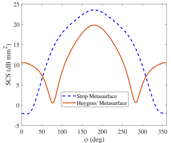
Fig. 9: Comparison of SCS of covered cylinders with strip metasurface and HMS versus \phi .
