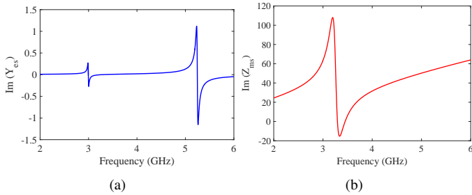
Fig. 5: Simulated (a) electric sheet admittance and (b) magnetic sheet impedance.
