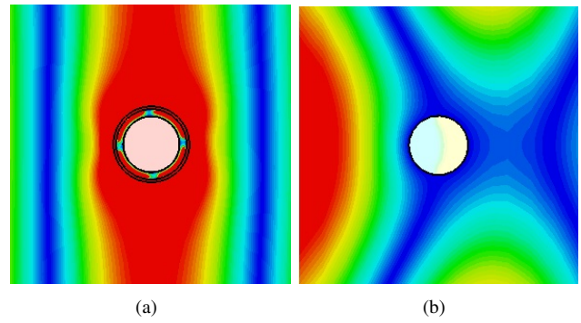
Fig. 8: Total electric field distribution around (a) cloaked and (b) uncloaked cylinders at 4 GHz.
