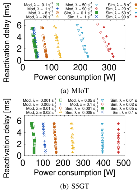
Fig. 10: Reactivation delay and average power consumption derived from the model (Mod) and via simulation (Sim) under multiple combinations of SM settings (different SM2 durations), in MIoT and S5GT scenarios.
