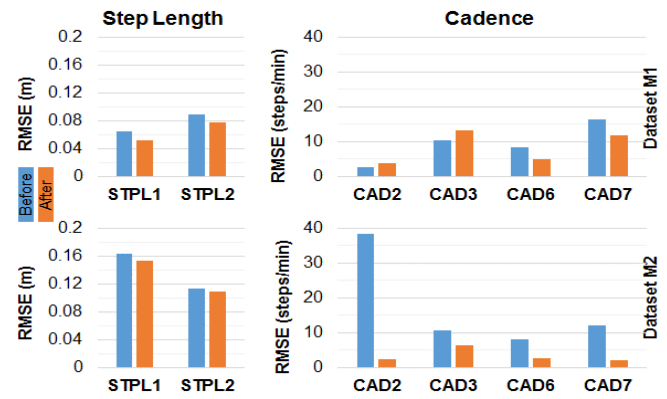
Fig. 4. RMSE of the algorithms before (blue) and after (orange) improvement, for step length (left side) and cadence (right side). The graphs in the upper panel show the results on dataset M1, and the lower panel for M2. The algorithms were trained (if required) and tested on ALL category of the train and test sets.
