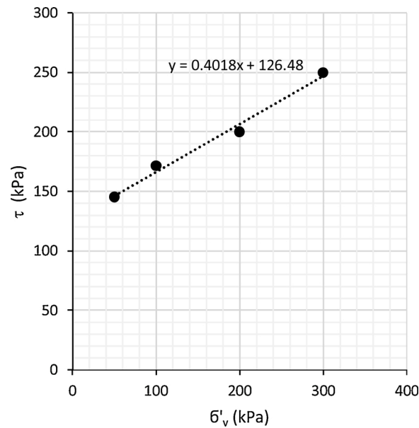
Fig. 12. Mohr-Coulomb failure criteria envelope pertaining to two-component grout samples cured for 3 h.
