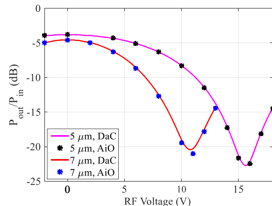
Figure 11. P_{\text{out}}/P_{\text{in}} characteristics obtained with the AiO full 3D FDTD simulations (markers) and with the DaC approach (solid lines) presented in this work for two modulators with L = 5 and 7 \mu\text{m} .
