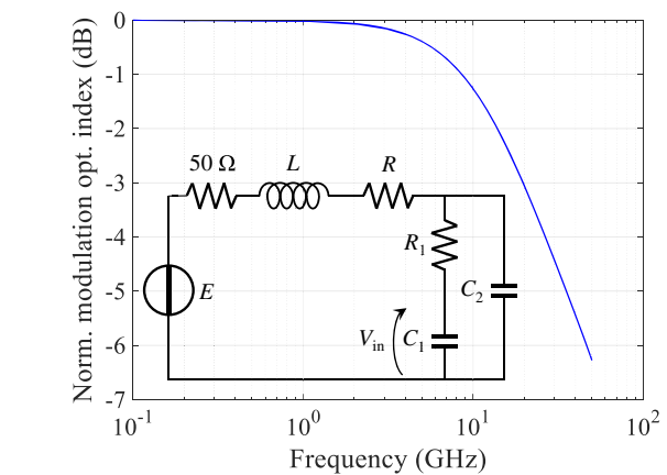
Figure 8. Frequency response of the modeled SOH MZM evaluated with the one-cell equivalent circuit shown in the inset. The assumed modulator length is 300 \mu\text{m} . The equivalent circuit parameters L and R are frequency dependent according to the results of the quasistatic model (see Figure 7). R_1 = 200 \Omega , C_1 = 62 \text{ fF} , and C_2 = 12.4 \text{ fF} .
