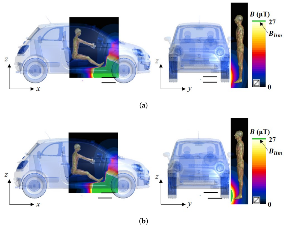
Figure 6. B-field distributions for the aligned (a) and misaligned (b) coil positions with the Al chassis.
