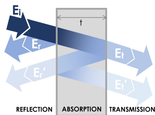
Figure 2. Mechanisms of attenuation of an electromagnetic radiation of energy E_i , incident on a shielding layer of thickness t : reflection, multiple reflections, and absorption. E_r(E_t) is the reflected (transmitted) energy, and E_r'(E_t') is the energy reflected (transmitted) after multiple crossing the layer. Color attenuation represents attenuation of energy.
