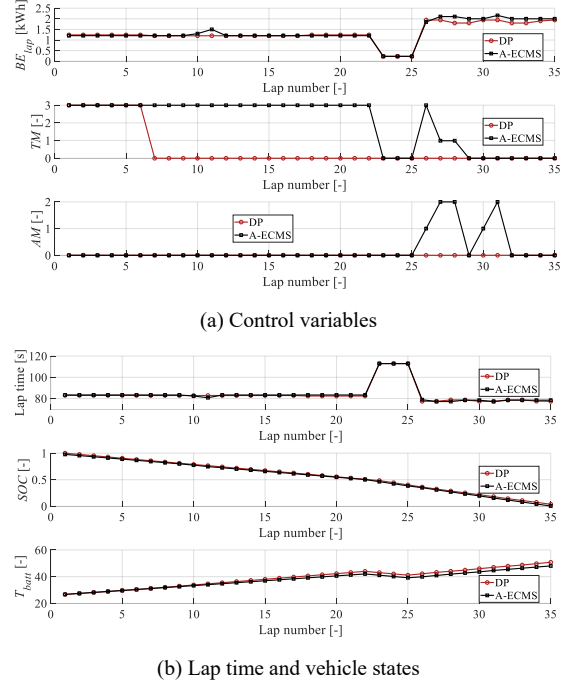
Fig. 10. Selected values of control variables, lap time and Formula E® car states as a function of lap number for both DP and A-ECMS (initial T_{batt} = 26^\circ \text{C} , safety car in lap 23 to lap 25).
