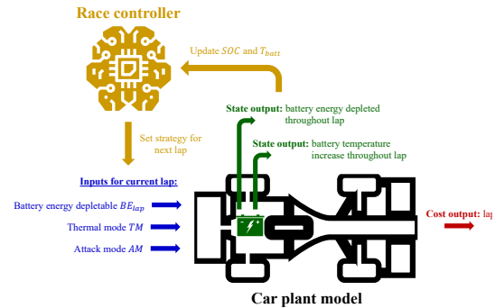
Fig. 1. Schematic diagram of the reduced-order plant model for a Formula E® car.
