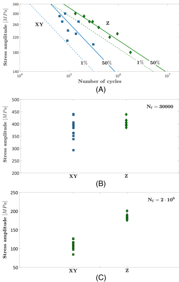
FIGURE 8 Experimental results obtained in Meneghetti et al. 33 : (A) S - N plot of the experimental dataset and estimated PSN curves; (B) stress amplitude with respect to the building direction for N_f = 30,000 cycles; (C) stress amplitude with respect to the building direction for N_f = 2 \cdot 10^6 cycles [Colour figure can be viewed at wileyonlinelibrary.com ]
