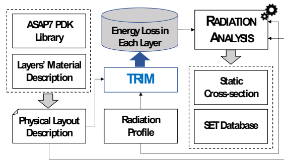
Fig. 2. The developed workflow for characterization of SET on 7 nm FinFET technology.
