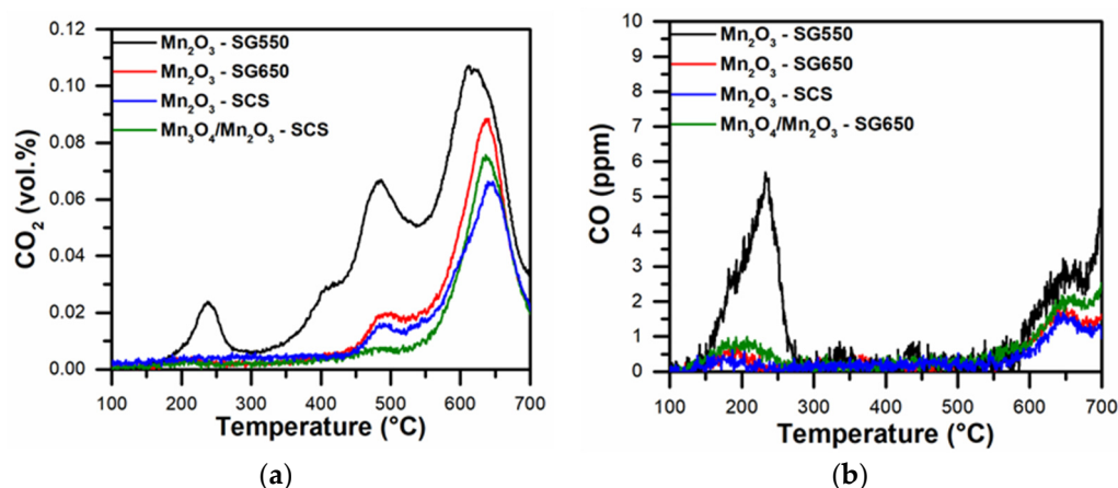
Figure 4. (a) \text{CO}_2 and (b) CO profiles observed during the soot-TPR analyses of the prepared catalysts.
