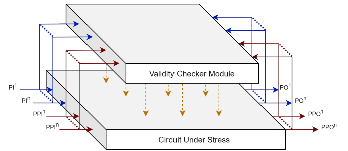
Fig. 3. Validity Checker Module interaction with the Circuit Under Stress
