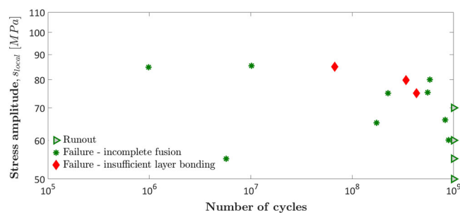
FIGURE 9 Stress-life (S-N) plot of the experimental data obtained considering s_{local} from in Paolino 42 [Colour figure can be viewed at wileyonlinelibrary.com ]
