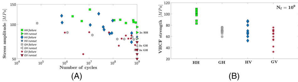
FIGURE 11 (A) Stress-life (S-N) plot of the experimental data obtained considering S_{local} and (B) estimated VHCF strength at 10^9 cycles from Tridello et al 44 [Colour figure can be viewed at wileyonlinelibrary.com]
