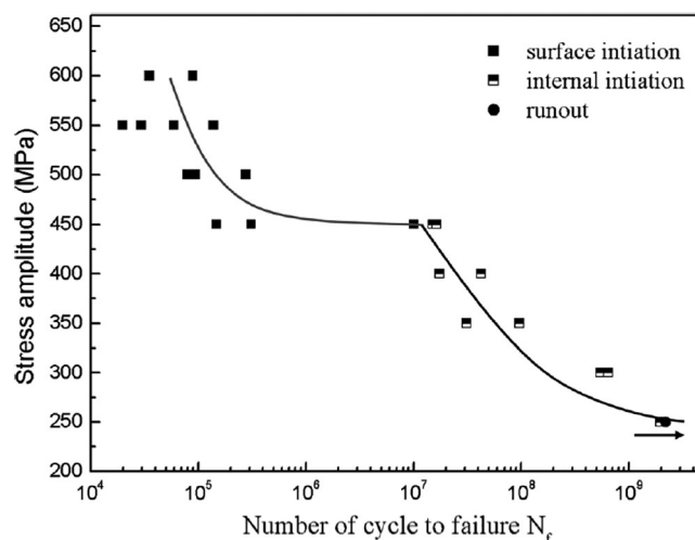
FIGURE 21 Stress-life (S-N) plot of experimental data from Liu et al. 63
