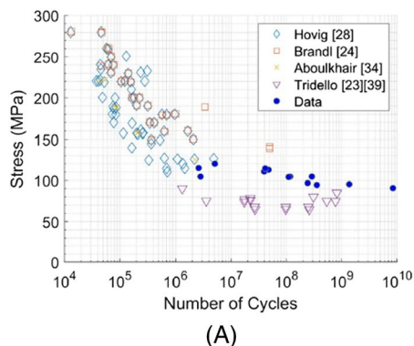
FIGURE 14 S-N plot of (A) AlSi10Mg batch compared with literature AlSi10Mg heat-treated data and (B) AlSi7Mg batch compared with literature cast AlSi7Mg data from Lesperance et al. 50 Note: The legend in the plot link to literature VHCF data which are in this paper renumbered as Tridello et al. 43 (Yamashita et al. 23 in the plot) Tridello et al. 40 (Tridello et al. 39 in the plot). For the other references about HCF data, the reader is referred to Lesperance et al. 50 [Colour figure can be viewed at wileyonlinelibrary.com ]
