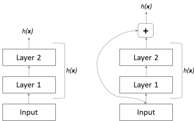
Fig. 13 Skip connection
