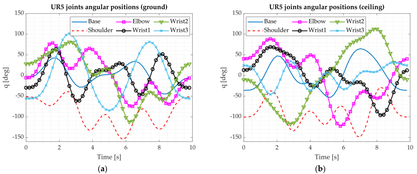
Figure 2. (a) Excitation trajectory for a UR5 collaborative robot mounted on the ground; (b) Excitation trajectory for a UR5 collaborative robot mounted on the ceiling.
