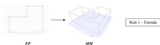
Figure 9. Rule 1 - extrudes a building footprint.
