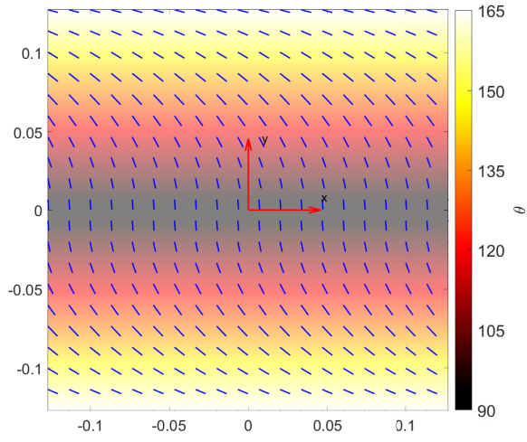
Figure 7: Case II [90 + \langle 0, 75 \rangle] fibre path. The fibre orientation angle \theta [deg] is measured with regard to the x -axis.
