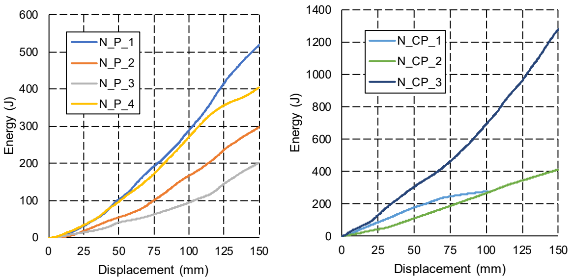
Figure 10: Absorbed energy-displacement curves obtained in the crushing tests on the impact attenuators.
