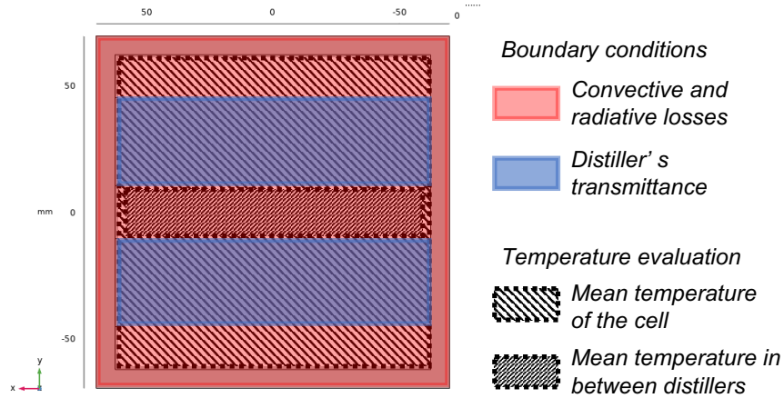
Figure S6: Bottom surface of the simplified FEM model. Convective and radiative losses are applied on the red area, while the thermal transmittance of the distillers on the blue area. The mean temperature of the PV cell is obtained by calculating the average temperature over the 125 \text{ mm} \times 125 \text{ mm} surface with large dashed lines. The mean temperature between the distillers is obtained calculating the average temperature over the surface with narrow dashed lines.
