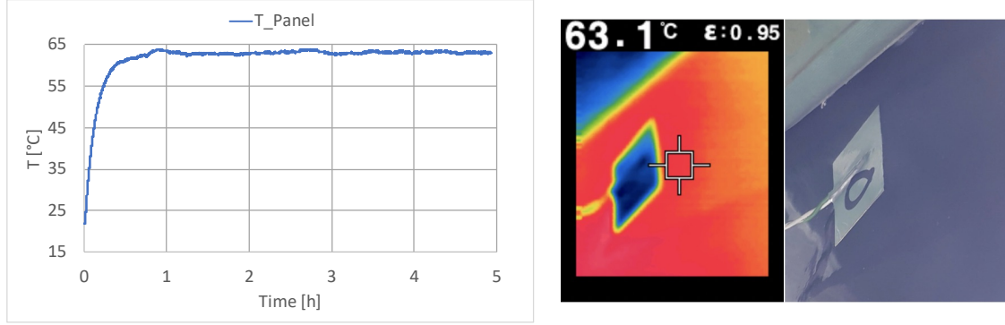
Figure S5: Emissivity characterization: temperature profile during the test (left); infrared and visible light pictures of a thermocouple placed on the panel (right).
