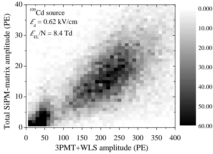
Figure 11: Direct SiPM-matrix readout: correlation between the amplitude of the total SiPM-matrix and 3PMT+WLS signals
