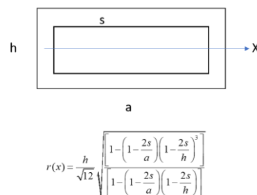
Figure 6b: Single rectangular thin-walled box and radius of inertia determination.
