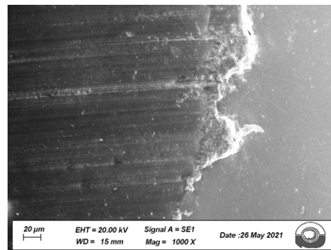
Figure 12. Detail of the edge of wear scar on ball after testing (Test 4).
