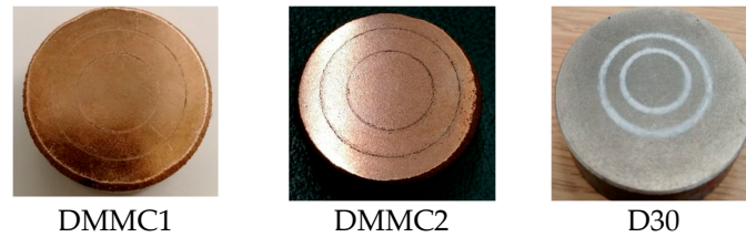
Figure 9. Wear scars on disks after test.
