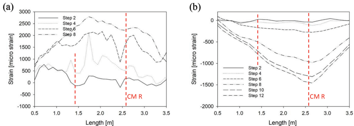
Fig. 13—Strain measures: (a) FOS at bottom concrete bulk of Beam 2; and (b) steel reinforcements at top of Beam 1. (Note: CM R is constant moment region.)
