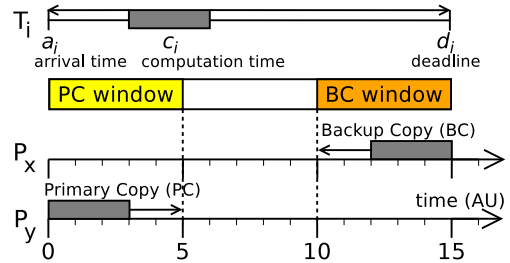
Fig. 5: PB approach with restricted scheduling windows ( f = 1/3 )
