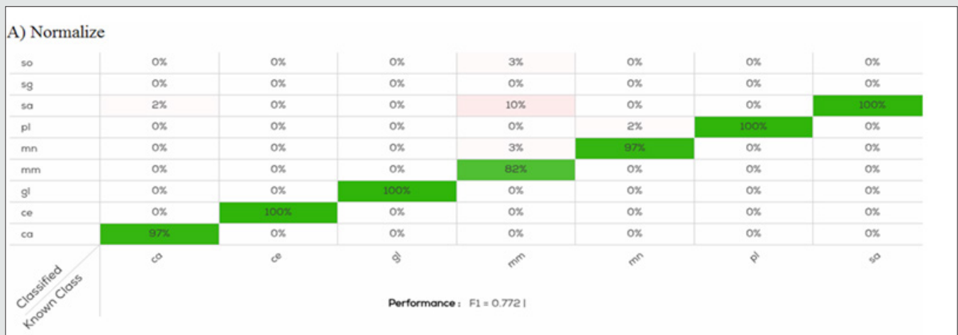
Figure 2A: Confusion table of Normalize model applied on calibration set. As showed Merluccius merluccius (mm) was the species with the lowest accuracy respect to the other one.
