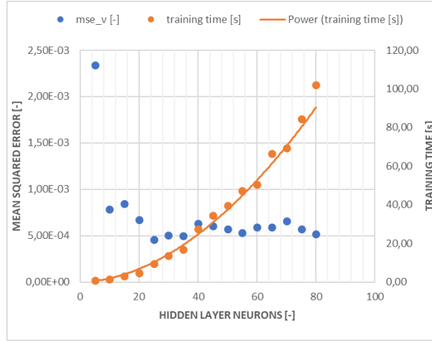
Figure 6: mse and training time with variation in the neurons number
