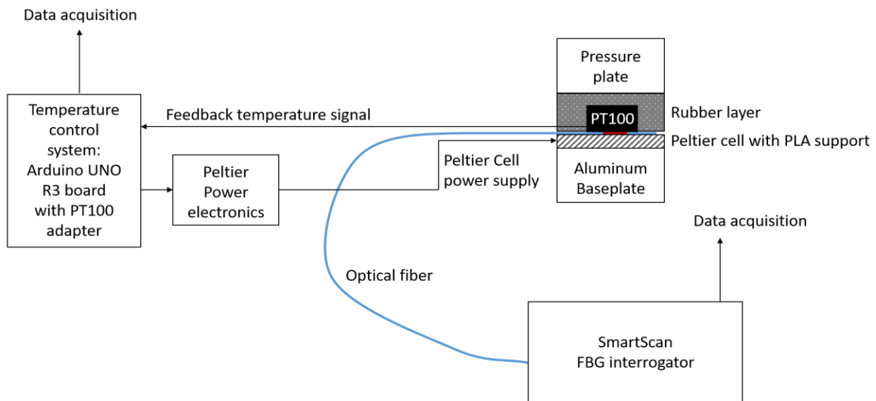
Figure6: Experimental setup for thermal tests.
