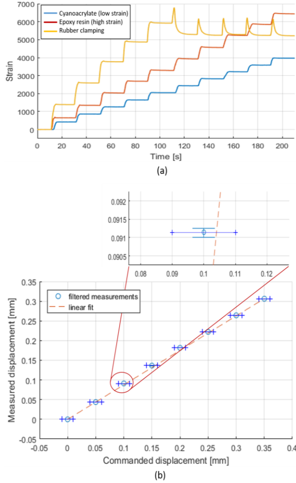
Figure 2: (a) comparison between rubber clamping of the fiber and gluing with cyanoacrylate and epoxy resin. (b) comparison between measured and imposed displacement.
