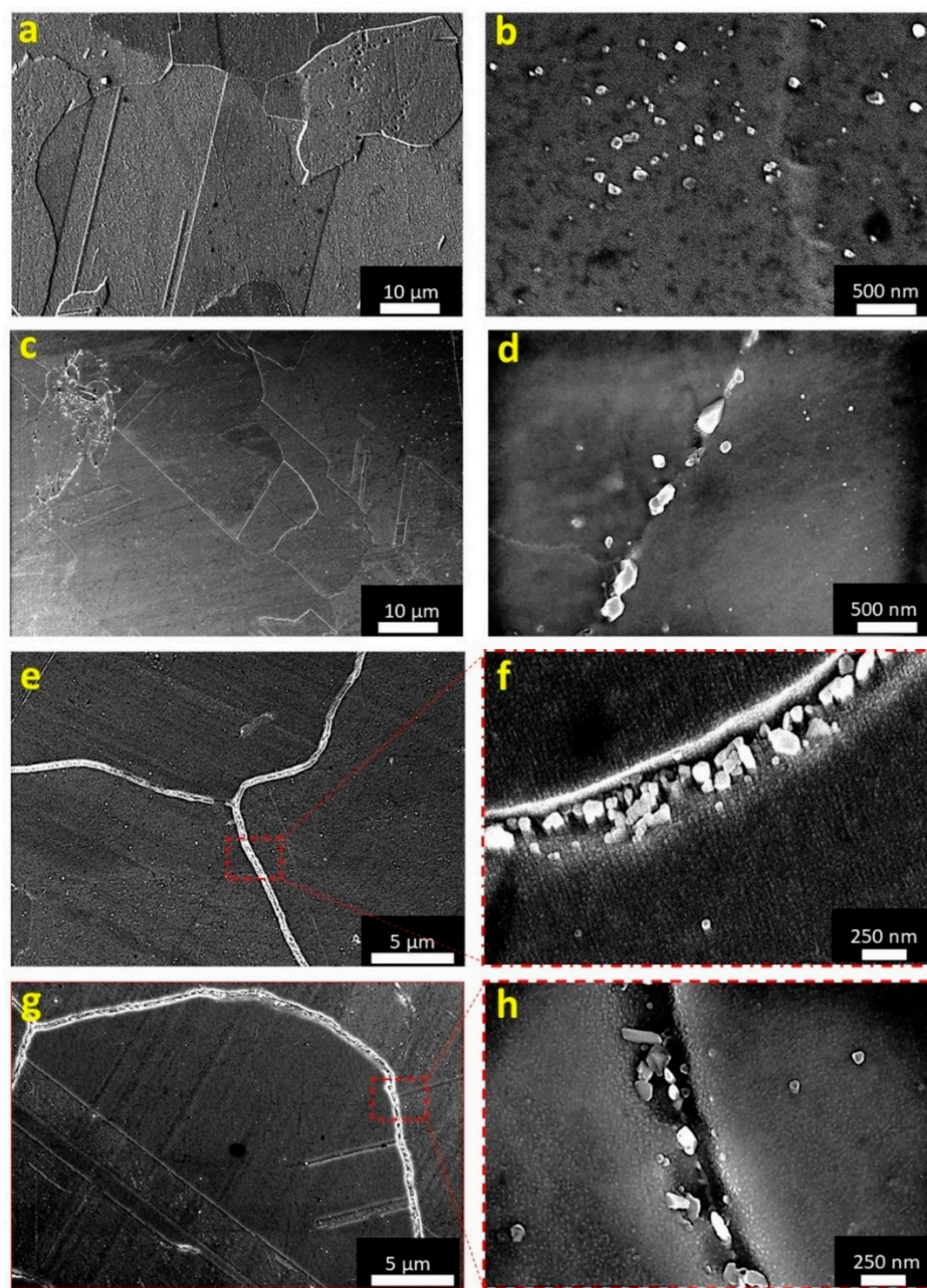
Figure 6. SEM images of the ST IN625 (a,b), ST IN625mod (c,d), STA IN625 (e,f), and STA IN625mod (g,h) showing the precipitates.
