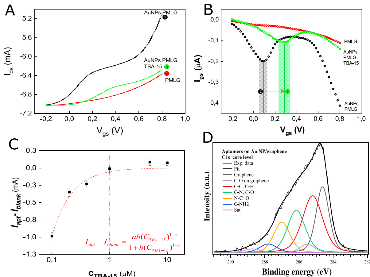
Figure 2. (A) comparison between the transfer curves for the different gate electrodes (i.e. unfolded TBA15-functionalized AuNPs-PMLG gate electrode (concentration 1 \mu\text{M} —green lines), bare PMLG (red lines) and AuNPs-PMLG (black lines)) and (B) related gate currents. Relative peaks are indicated with (2) for the AuNPs-PMLG and (3) for TBA15-functionalized AuNPs-PMLG gate electrode; (C) Optimization of the I_{\text{apt}} - I_{\text{blank}} parameter as a function of the aptamer concentration (fitting curve: Langmuir isotherm, red line); (D) C1s core level XPS analysis of PMLG/AuNPs/TBA-15. Single components are described in the legend.
