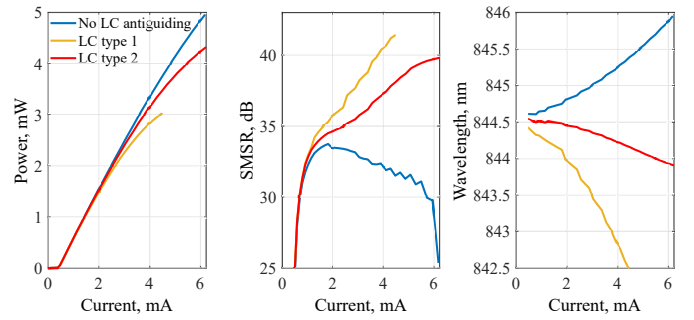
Fig. 10. LC-VCSEL performance vs. LC antiguinding features: LI, SMSR and lasing wavelength for a 4 \mu\text{m} oxide aperture, n_e=1.63 , 3 \mu\text{m} reservoir, 600 nm SU-8 and ambient temperature of 300 K.
