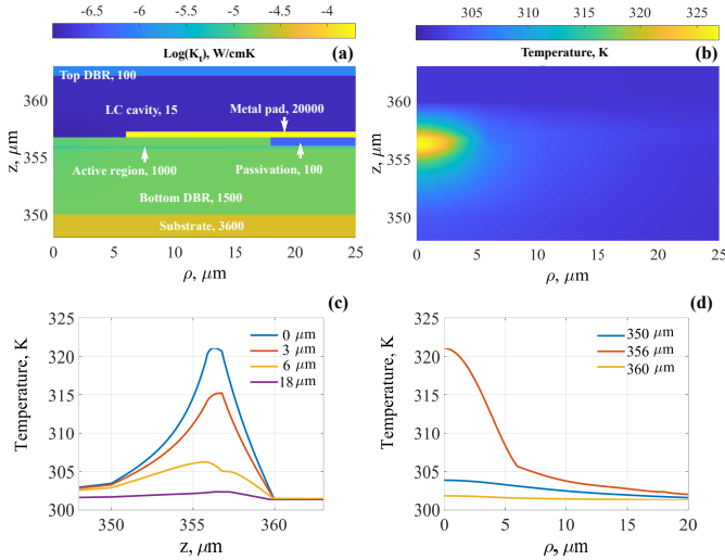
Fig. 9. (a) Map of the thermal conductivity ( \rho -z cut) and (b) corresponding thermal profile for a 4 \mu\text{m} VCSEL with n_e = 1.63 and I=5 mA around the active region. Thermal conductivity values (in W/cmK) are indicated by white labels, on the (a) map where the different regions are identified. For semiconductor see [?], for glass, top-DBR and for LC see [?]. (c) longitudinal temperature cuts at different radii (see legend); (d) transverse temperature cuts at different longitudinal sections. z=0 correspond to the heatsink, below the 350 \mu\text{m} substrate.
