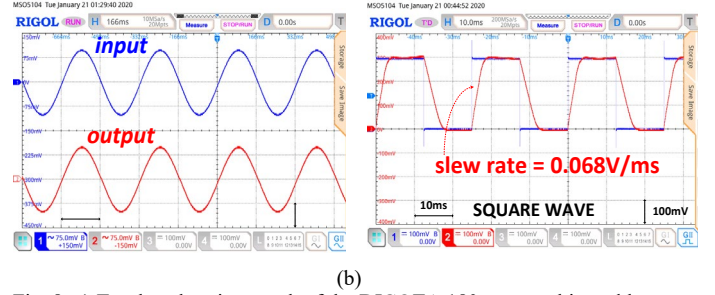
Fig. 8. a) Test bench, micrograph of the DIGOTA 180-nm testchip and layout, b) sine/square wave response when directly powered by a 1-mm 2 solar cell at <100 lux (dark overcast day) (2.5-Hz frequency, 75-mV amplitude).
