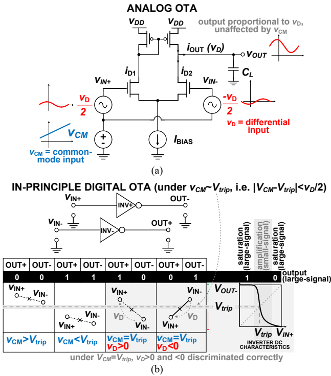
Fig. 1. In-principle schematic of a) analog OTA, b) digital OTA (DIGOTA). rejecting its common-mode component v_{CM} = (v_{IN+} + v_{IN-})/2 . The reliance of DIGOTA on logic gates inherently reduces the power floor imposed by bias currents and reference circuits necessary in conventional analog OTAs [11]-[14], [23], enabling power savings well beyond their analog counterparts.
